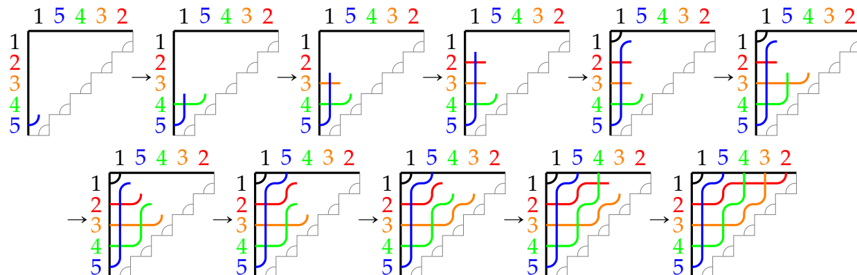
Figure 2: The sweeping algorithm with \omega = 15432 and \pi = 15243 .
