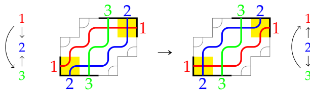
Figure 7: An increasing flip between two non-comparable acyclic pipe dreams.
