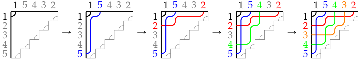
Figure 3: The insertion algorithm with \omega = 15432 and \pi = 15243 .
